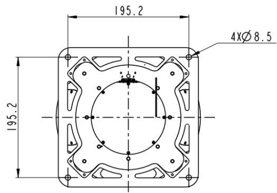
Picture 2 Product Dimensions
